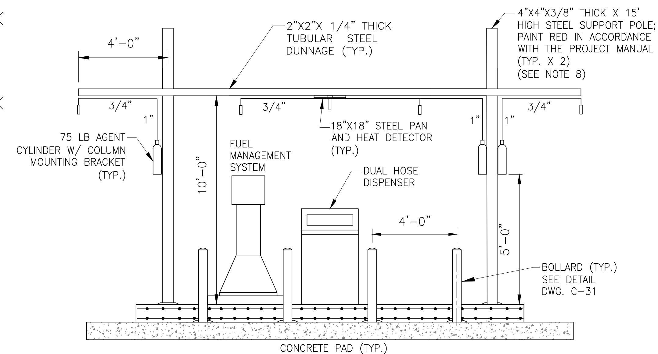
DUAL HOSE DISPENSER ISLAND ELEVATION
