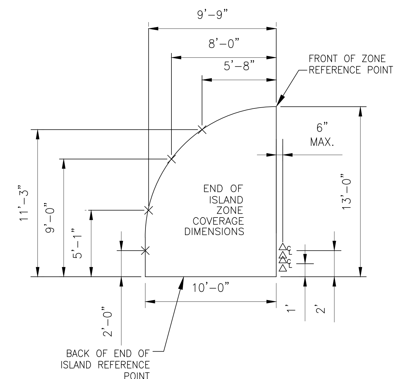
TYPICAL NOZZLE AIMING POINTS DETAIL
